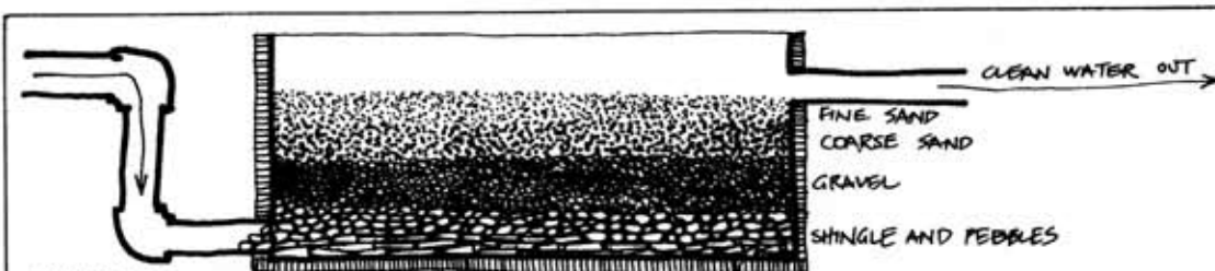
FIGURE 7.32 SAND FILTER
