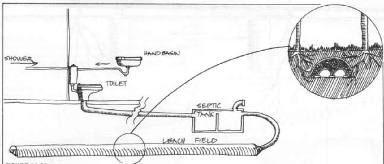
FIGURE 11.68 ARBOR SYSTEM.
