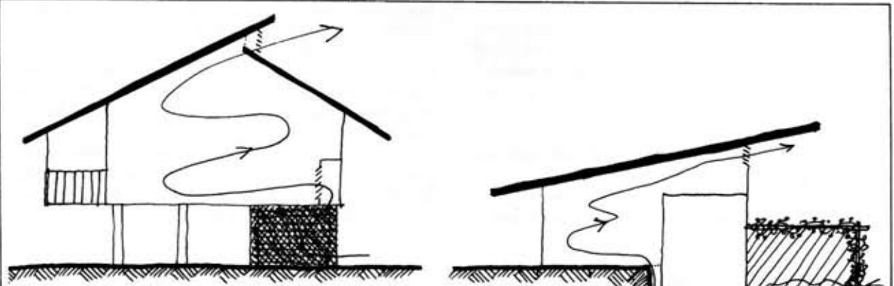
FIGURE 10.16 CROSS-VENTILATION FOR HOUSES Vented ceiling slopes allow hot room air to escape, and cool trellis air to enter.
