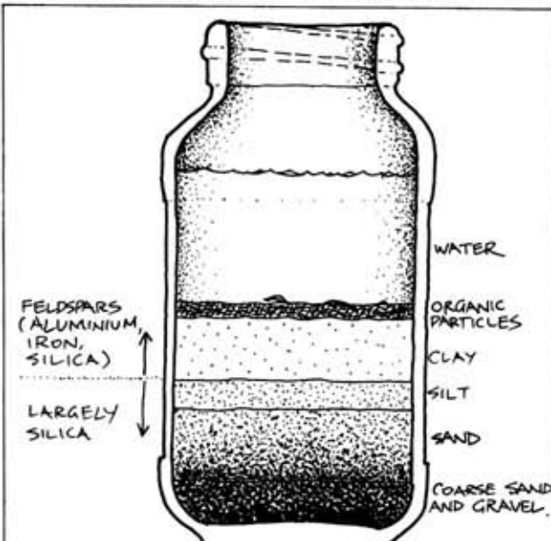
FIGURE 8.2 JAR METHOD
