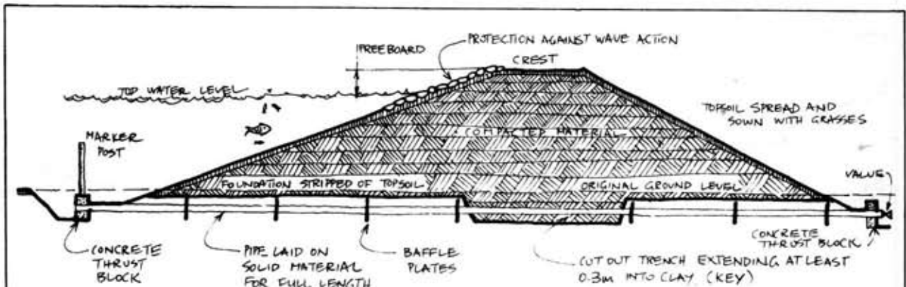
FIGURE 7.18 DAM WITH LOCK PIPES.
