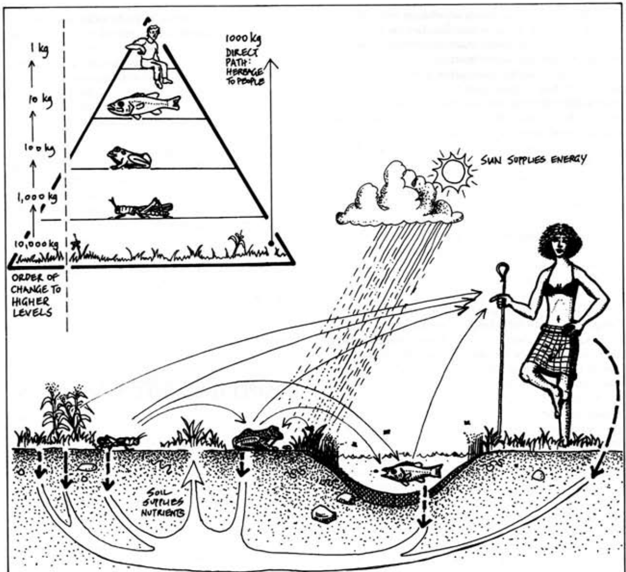
FIGURE 2.6 TROPHIC PYRAMID.
