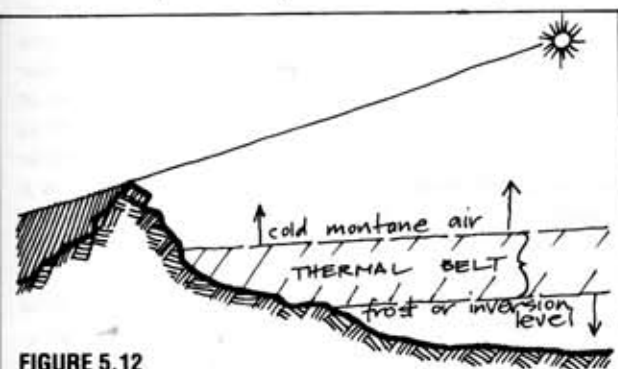
FIGURE 5.12 THERMAL BELT.
