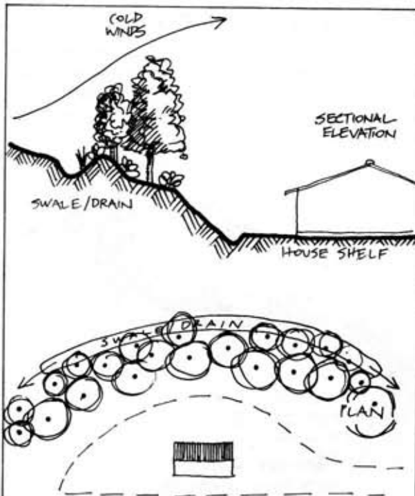
FIGURE 9.16 RAISED BANK BESIDE HOUSE In areas of heavy rains, house sites must be carefully designed to deflect downhill overland flow.
