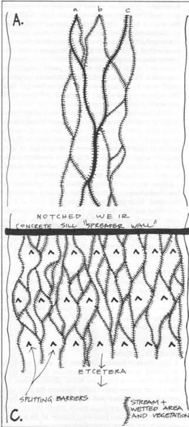
FIGURE 11.38. A BRAIDED STREAM. A natural braid occurs in sand beds at the centre of flood plains. B NOTCHED WEIRS can spread flood braiding across a full flood plain; hatched areas show absorption areas where trees and shrubs will grow (see detail). C. Details of braid patterns in sand, notched weir to initiate braiding in sandy rivers.
