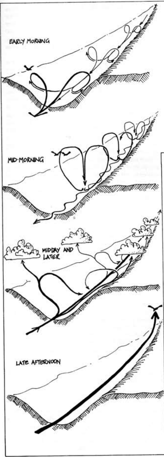
FIGURE 5.25 VALLEY WINDS
