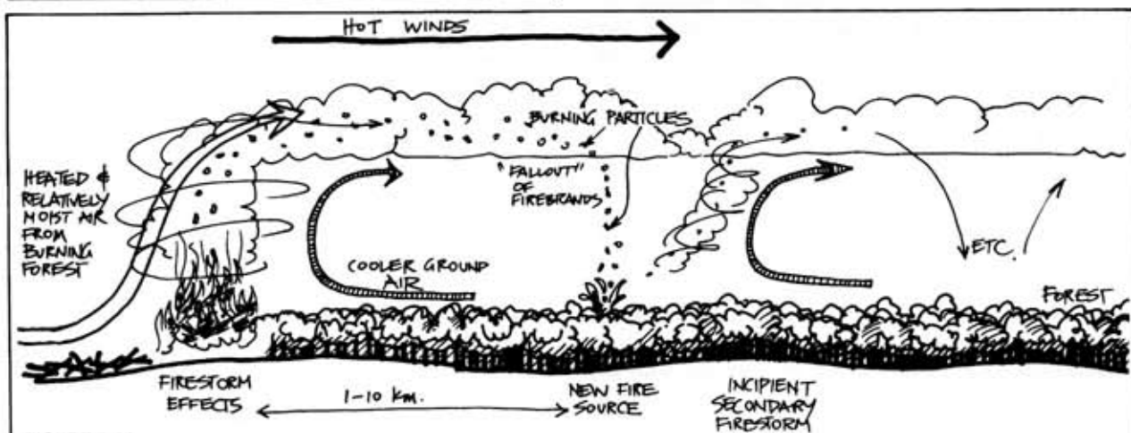
FIGURE 5.23 FIRESTORMS.
