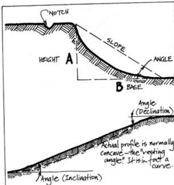
FIGURE 9.4 CONCAVE SLOPES
