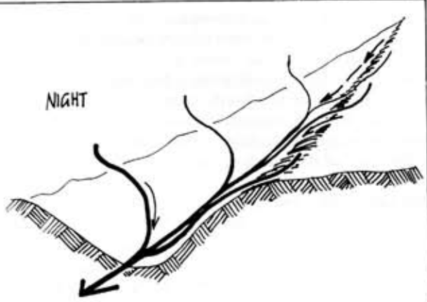
FIGURE 5.25 VALLEY WINDS
