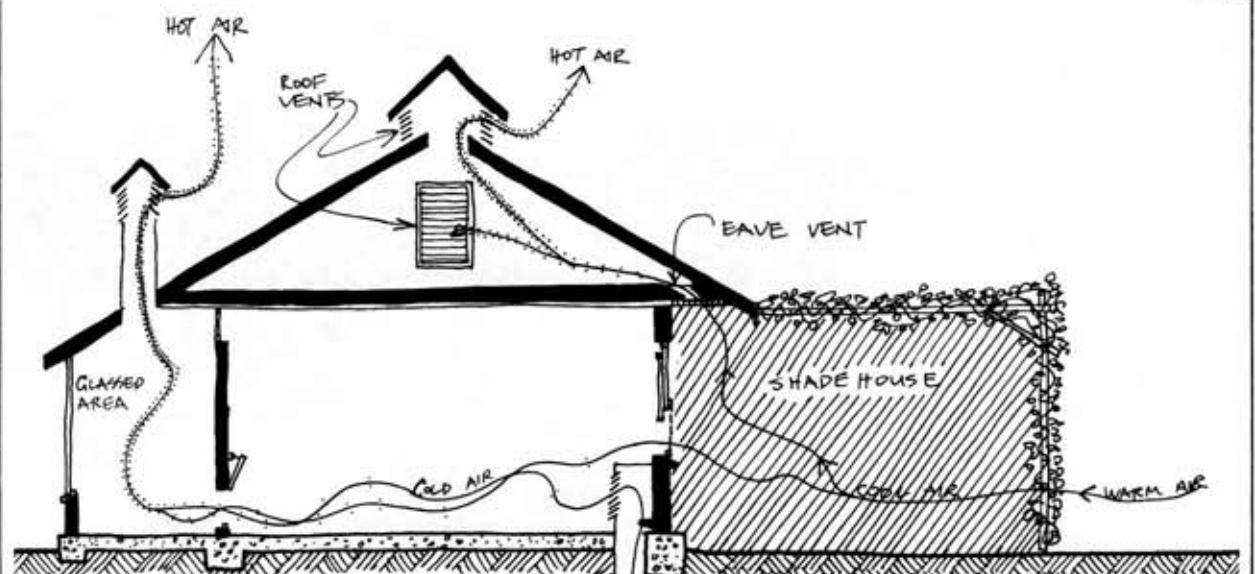
FIGURE 10.17 COOL AIR FROM SHADEHOUSE AND BURIED PIPE. A 0.5 x 0.5 m tunnel 1 m deep and 20 m long sloping to the outside intake to de-humidify and cool equatorial air, with a solar chimney to draw air through the house.
