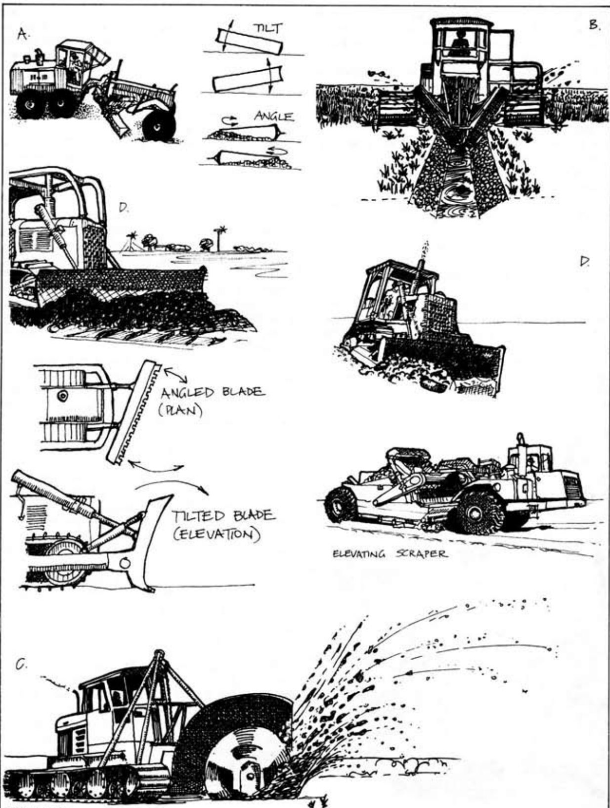
FIGURE 9.27 LARGE MACHINES; On many machines, tilt, angle, and lift blades enable accurate work on roads and drains. A selection of blades and systems are shown: A - grader, B - delver, C - spinner, D - bulldozer.
