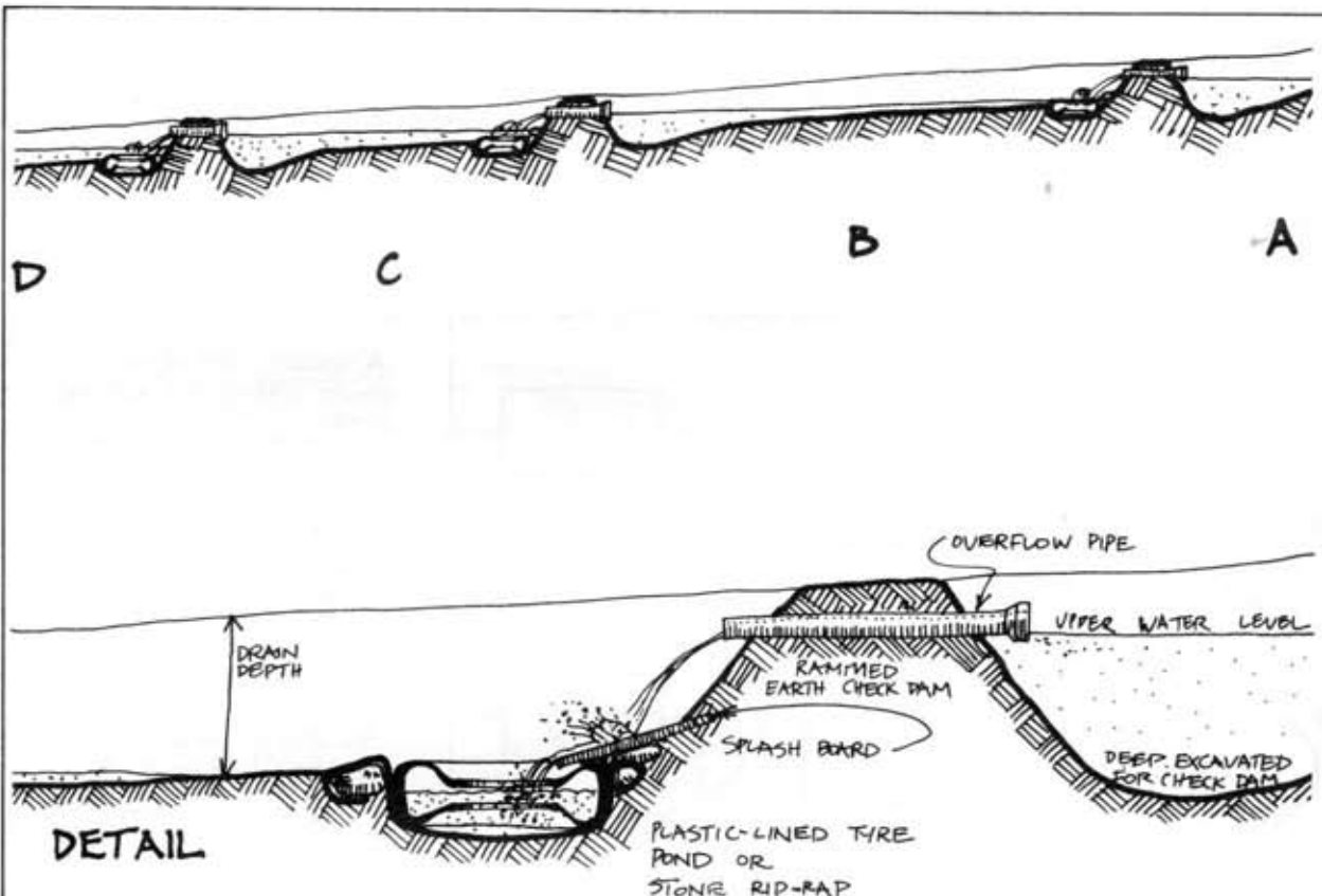
FIGURE 13.14 CONSECUTIVE SERIES IN OPEN DRAINS.
