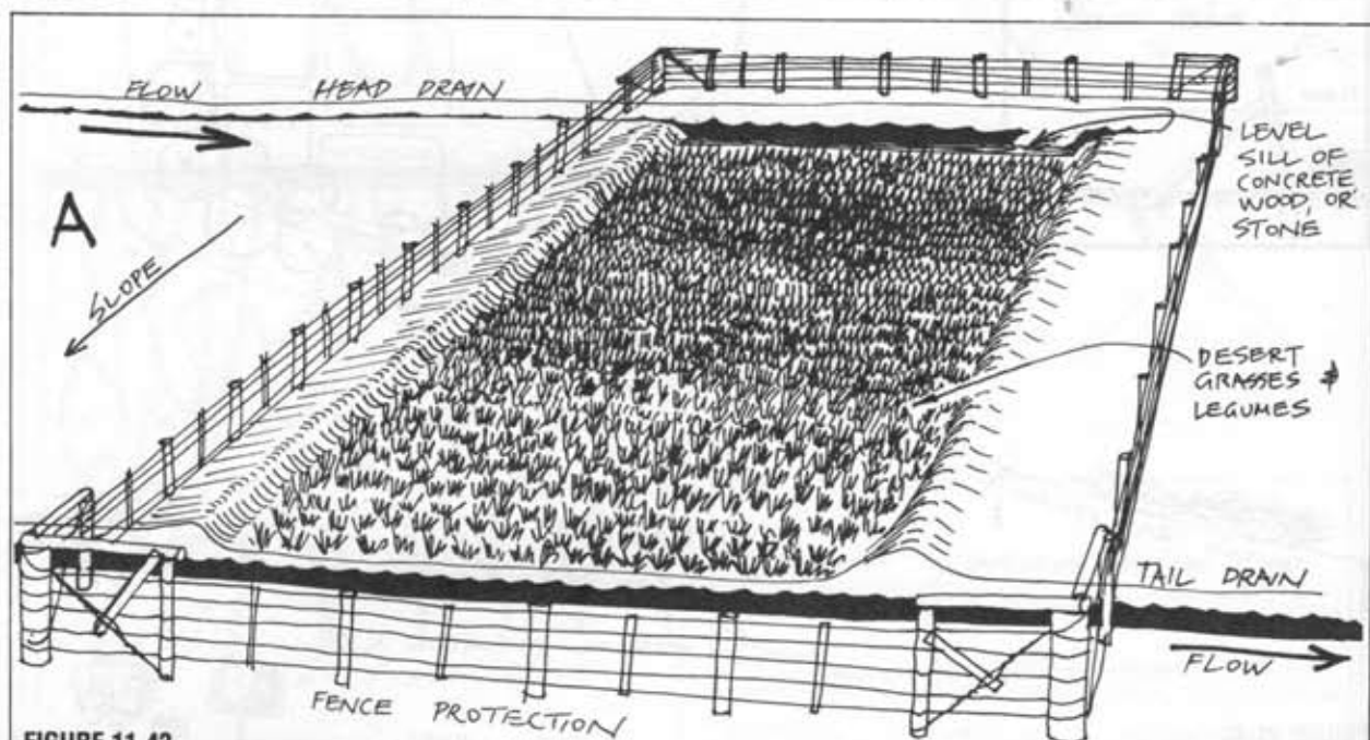
FIGURE 11.42 GRASSED SPILLWAYS WITH STEERING BANKS.
