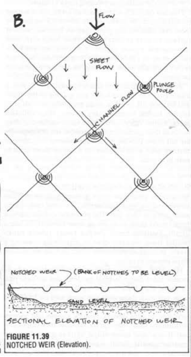
FIGURE 11.38. A BRAIDED STREAM. A natural braid occurs in sand beds at the centre of flood plains. B NOTCHED WEIRS can spread flood braiding across a full flood plain; hatched areas show absorption areas where trees and shrubs will grow (see detail). C. Details of braid patterns in sand, notched weir to initiate braiding in sandy rivers.
