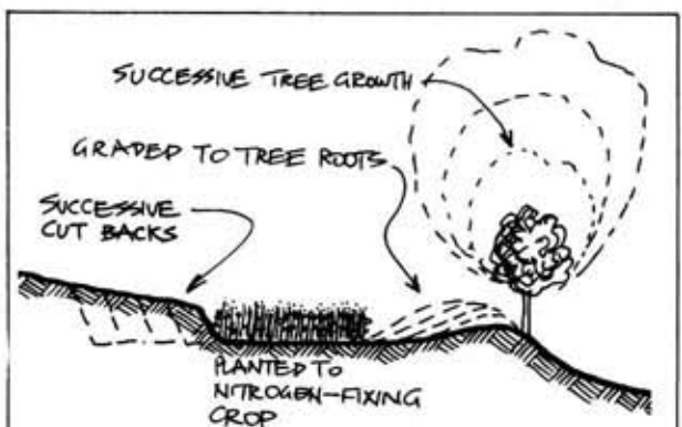
FIGURE 7.25 REGRAIDING SWALES TO REMOVE SILT
