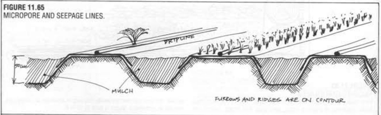
FIGURE 11.65 MICROPORE AND SEEPAGE LINES.
