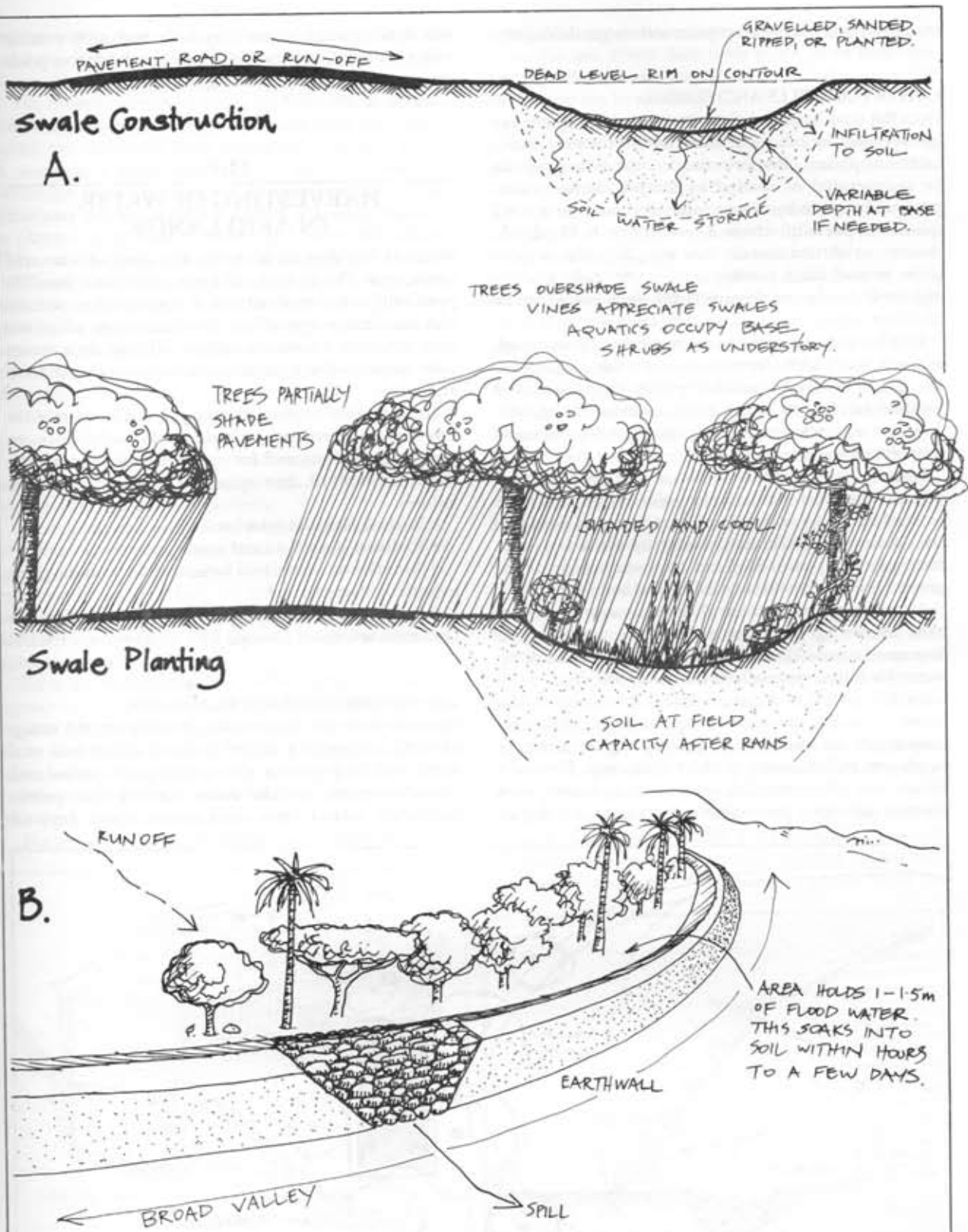
FIGURE 11.27 SWALE CONSTRUCTION.
