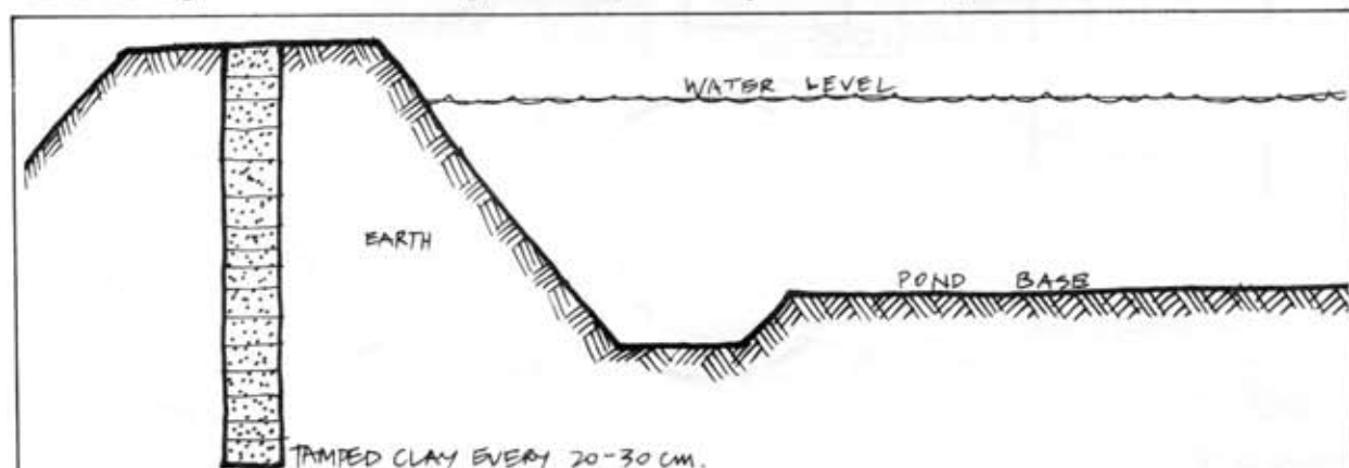
FIGURE 13.12 POND WALLS
