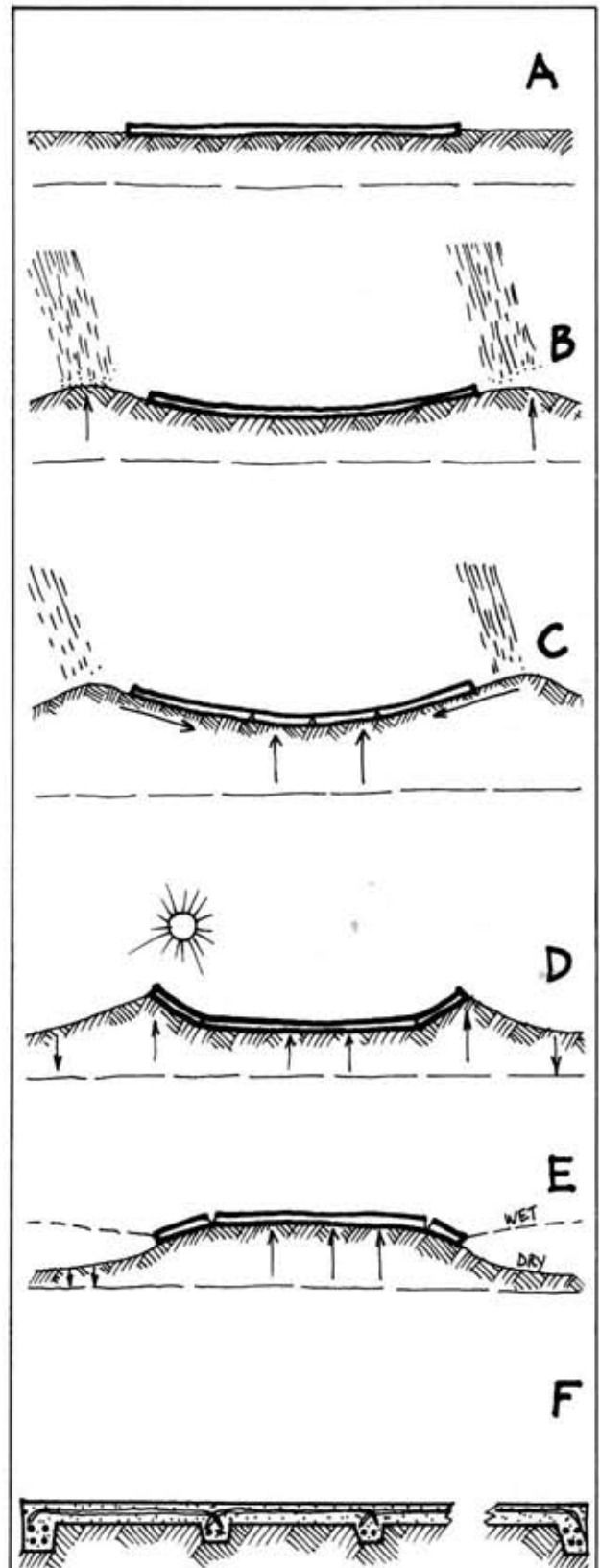
FIGURE 8.14 A–E HOW A MOUND DEVELOPS UNDER A HOUSE F Slab plus beam construction helps stability.
