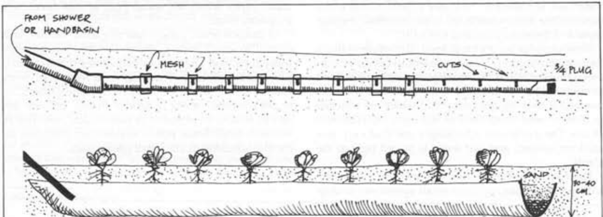
FIGURE 11.67 DOMESTIC WASTE WATER CHANNELS.
