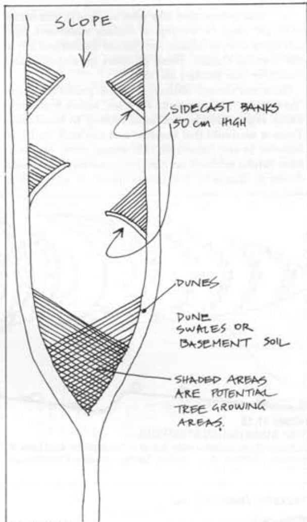
FIGURE 11.17 CHEVRON BANK IN DUNE SWALES. Side-cast banks halt flood flow down dune swales; hatched areas will grow trees (parallel dune series); swales so chosen must have a slope "downhill".
