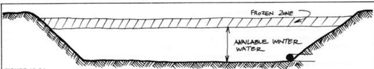
FIGURE 12.24 EXPANDING ICE IN WATER STORAGE. Sides of storages need to be sloped to allow for freeze expansion; capacity must be judged as unfrozen depth over winter.
