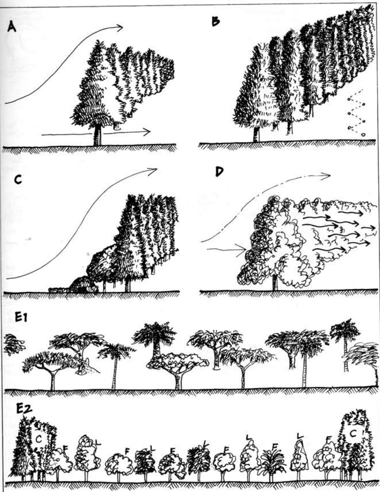
FIGURE 5.18 WINDBREAK CONFIGURATIONS.
