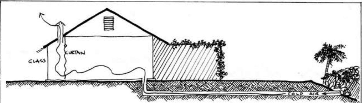
FIGURE 10.16 CROSS-VENTILATION FOR HOUSES Vented ceiling slopes allow hot room air to escape, and cool trellis air to enter.
