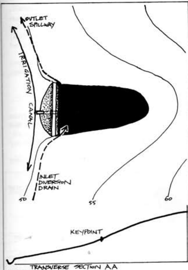
FIGURE 7.6 KEYPOINT DAM
