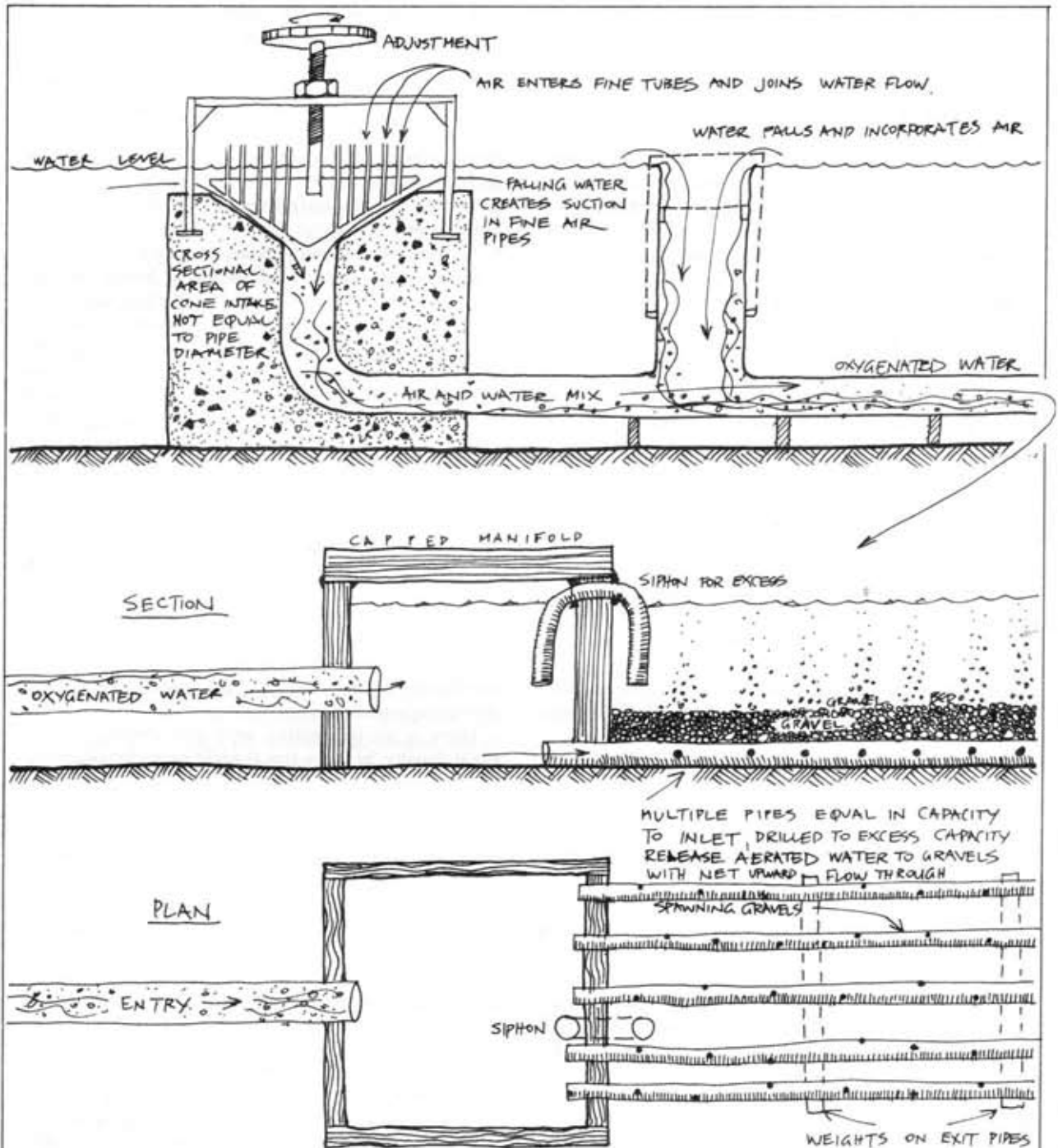
FIGURE 13.7 CONE AERATOR
