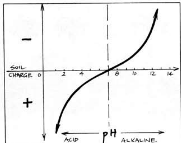
FIGURE 10.2 TROPICAL CLAYS
